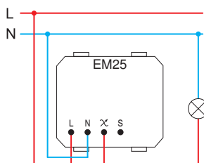
(2)lidhje me tre tela three-wire connection
